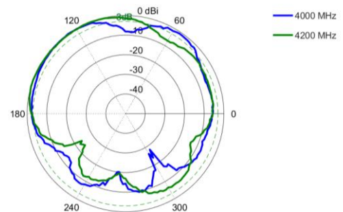
Azimuth: 4000 – 4200 MHz
