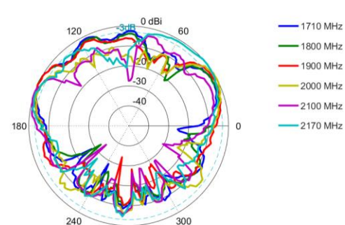
Elevation 1: 1710 – 2170 MHz
