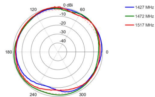
Azimuth: 1427 – 1517 MHz
