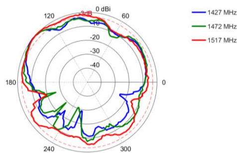
Elevation 1: 1427 – 1517 MHz
