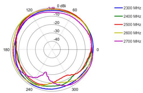
Elevation 2: 2300 – 2700 MHz
