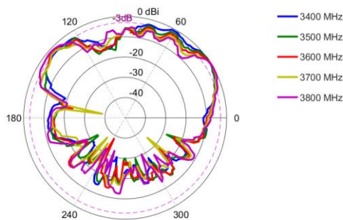
Elevation 2: 3400 – 3800 MHz
