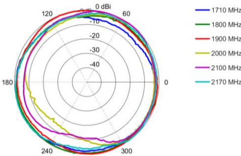
Azimuth: 1710 – 2170 MHz
