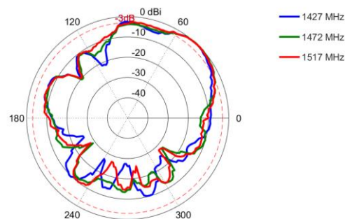
Elevation 2: 1427 – 1517 MHz
